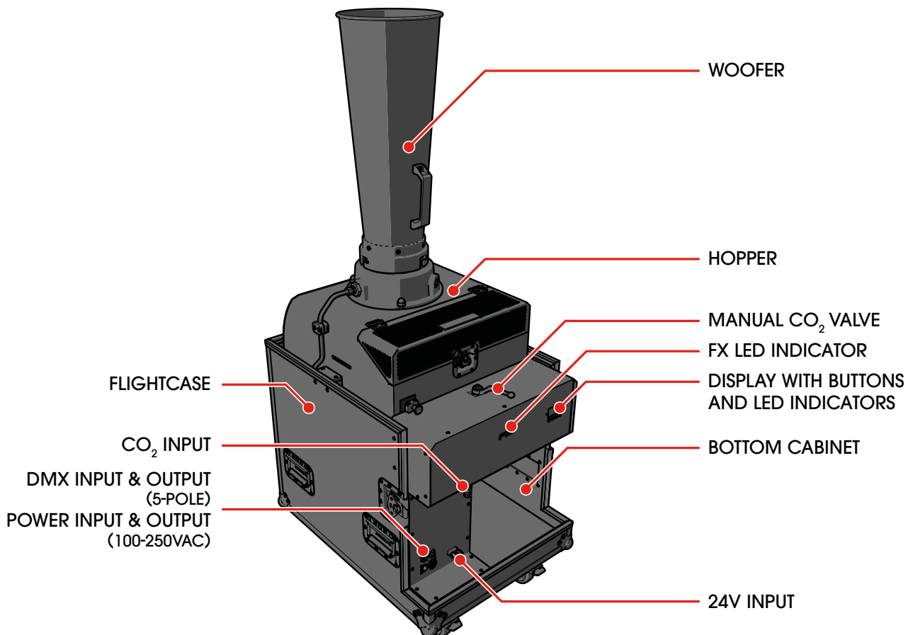
Main parts in backside view
